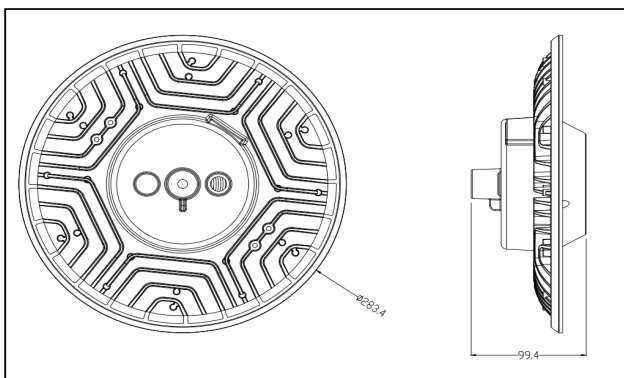
Physical dimension ( mm )
