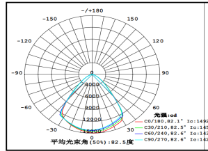
90° Optical
