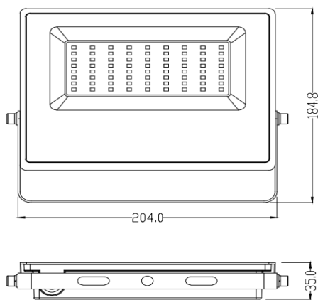
FG104-50W Physical dimension (mm)
